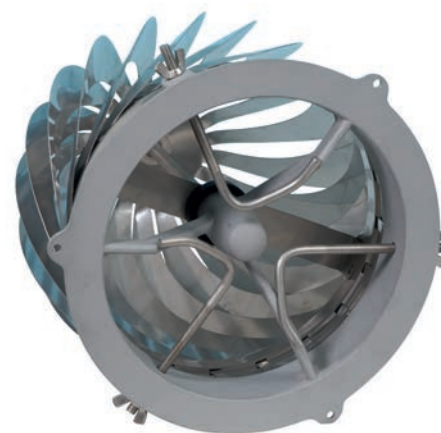
Base of the Turbolite showing greater surface area through which gasses may pass
